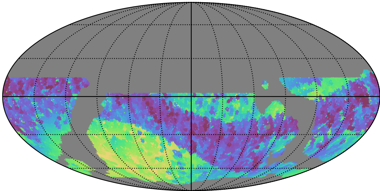
weather_cloudso4v3.4_10yrs WFD i band: Min skyBrightness
