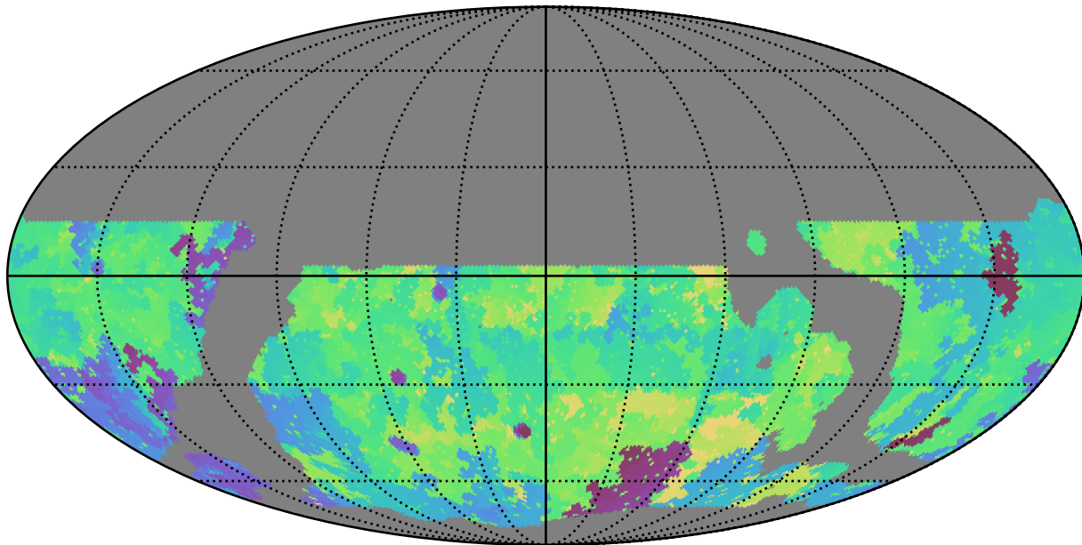
weather_cloudso4v3.4_10yrs WFD g band: Min skyBrightness
