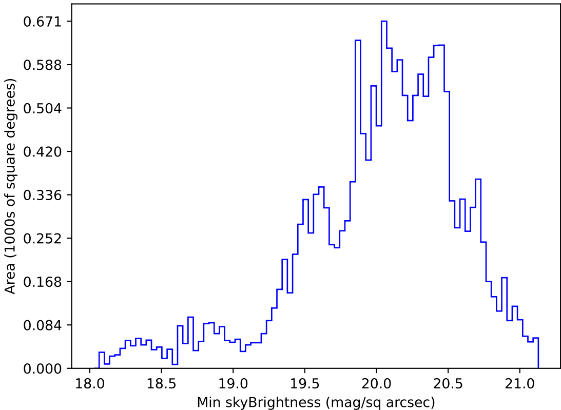
weather_cloudso4v3.4_10yrs WFD g band: Min skyBrightness
