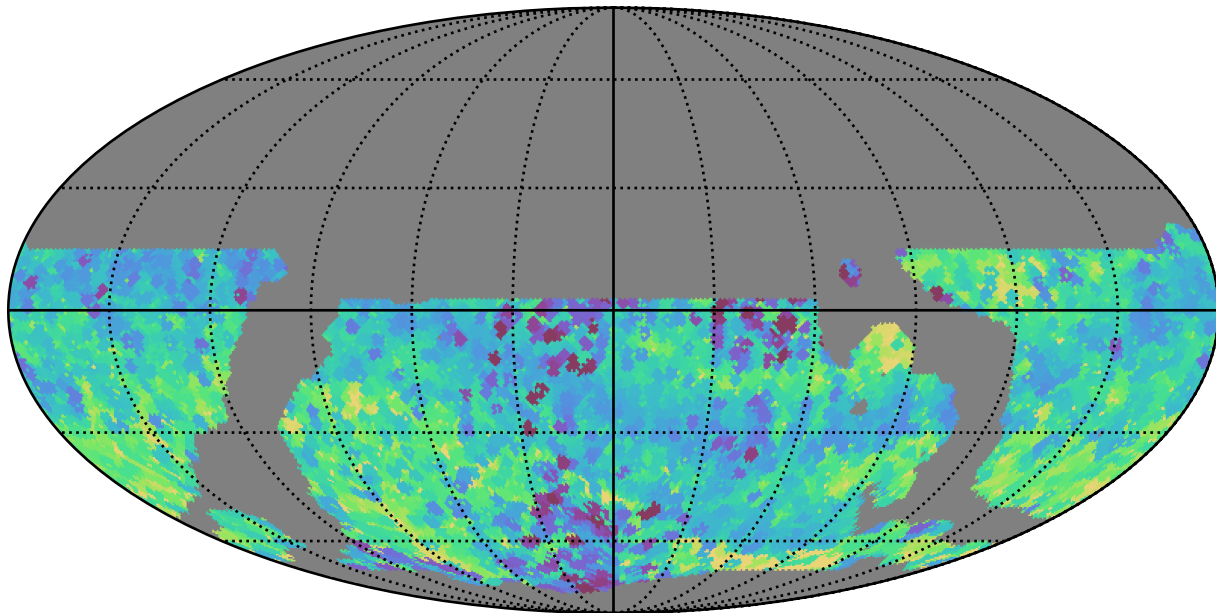
weather_cloudso4v3.4_10yrs WFD all bands: Min skyBrightness
