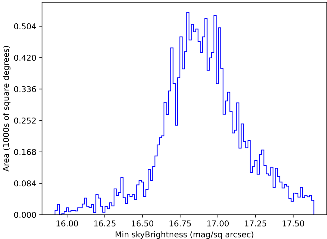
weather_cloudso4v3.4_10yrs WFD all bands: Min skyBrightness
