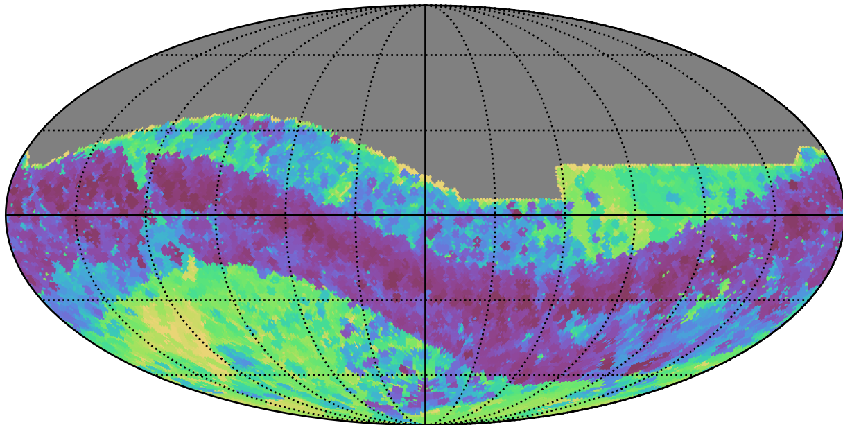
weather_cloudso4v3.4_10yrs All sky z band: Min skyBrightness
