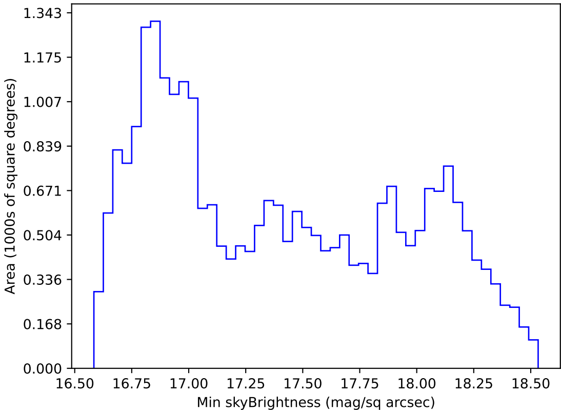
weather_cloudso4v3.4_10yrs All sky z band: Min skyBrightness
