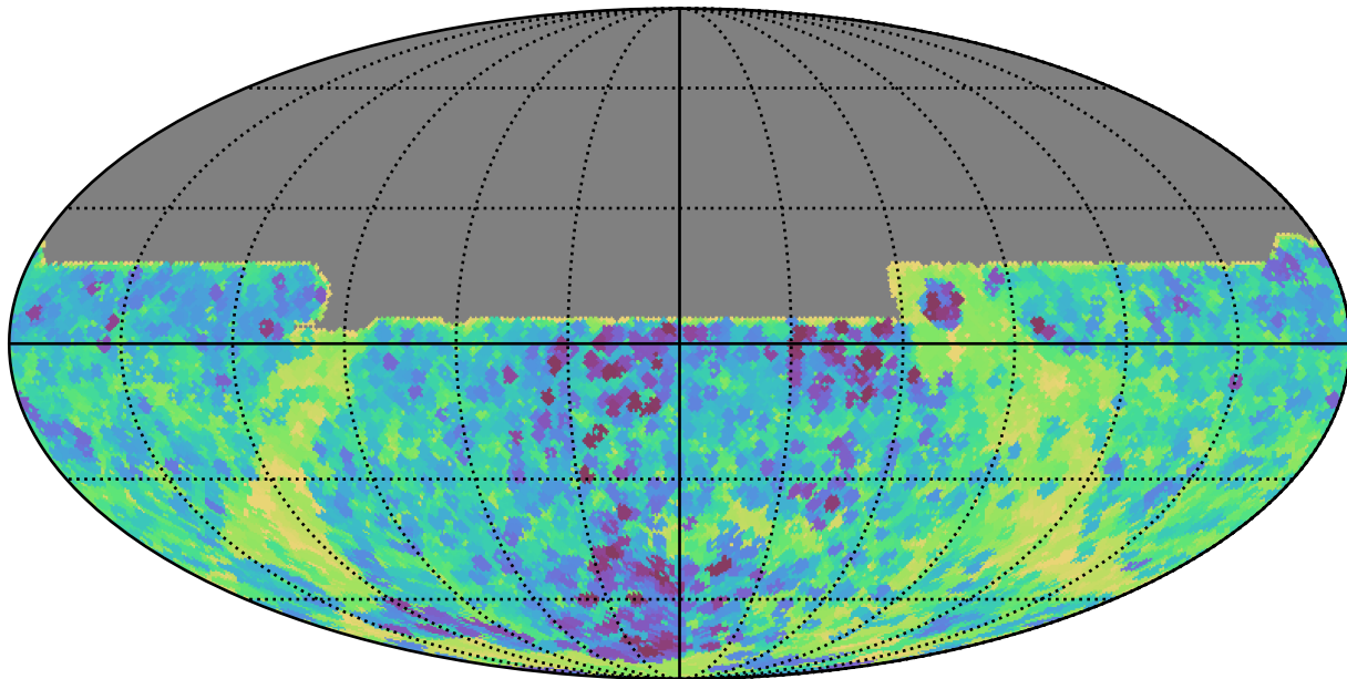
weather_cloudso4v3.4_10yrs All sky y band: Min skyBrightness
