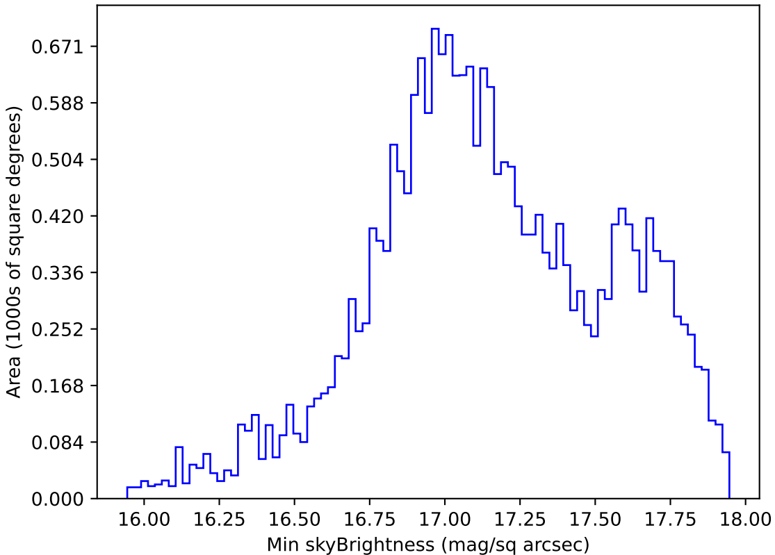
weather_cloudso4v3.4_10yrs All sky y band: Min skyBrightness
