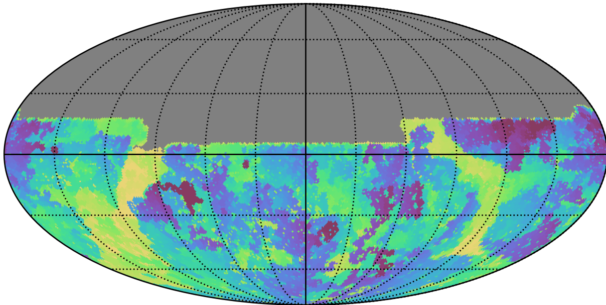
weather_cloudso4v3.4_10yrs All sky u band: Min skyBrightness
