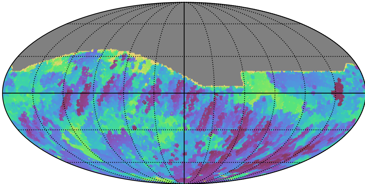
weather_cloudso4v3.4_10yrs All sky r band: Min skyBrightness
