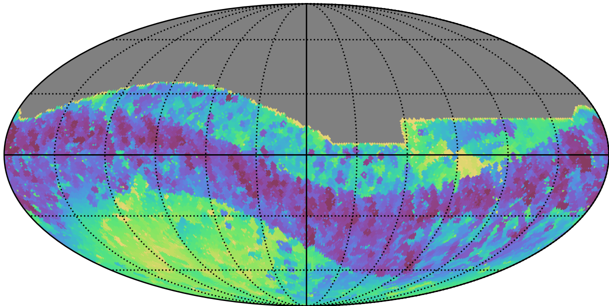
weather_cloudso4v3.4_10yrs All sky i band: Min skyBrightness
