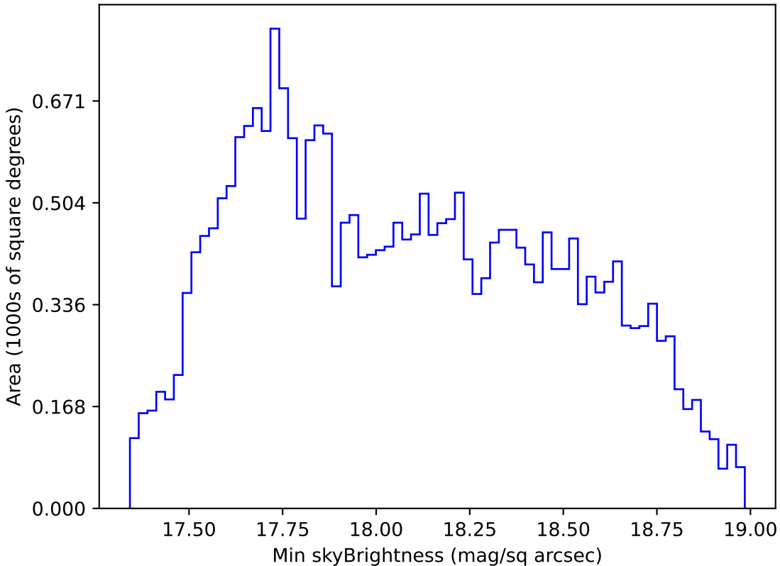
weather_cloudso4v3.4_10yrs All sky i band: Min skyBrightness
