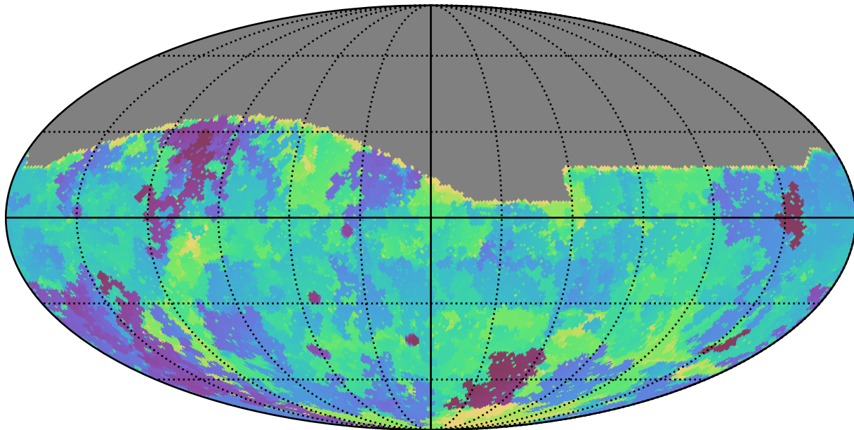
weather_cloudso4v3.4_10yrs All sky g band: Min skyBrightness
