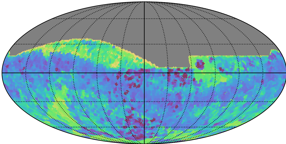
weather_cloudso4v3.4_10yrs All sky all bands: Min skyBrightness
