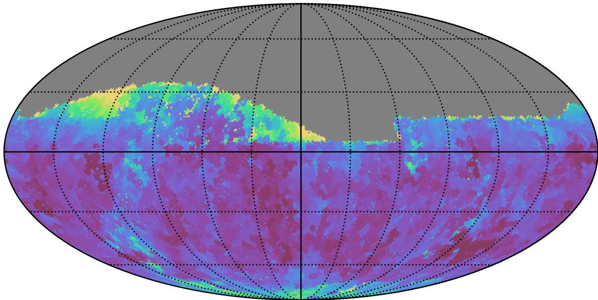
weather_cloudso4v3.4_10yrs Yr 1 z band: Min seeingGeom
