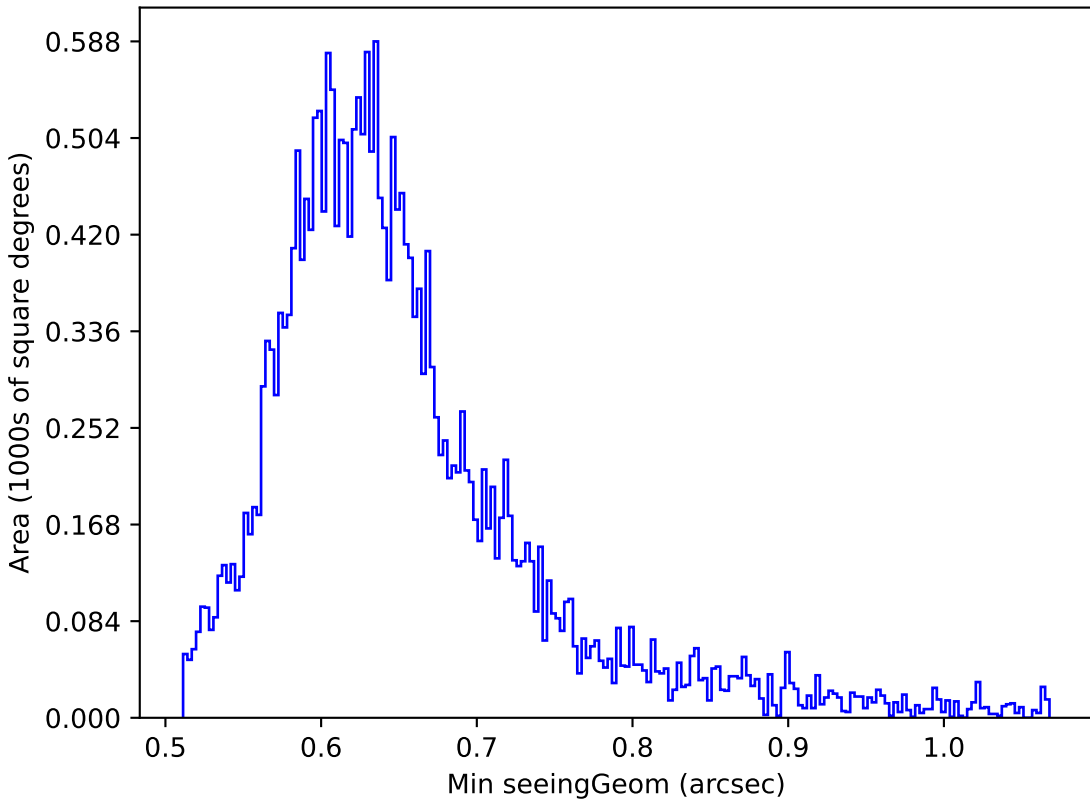
weather_cloudso4v3.4_10yrs Yr 1 z band: Min seeingGeom
