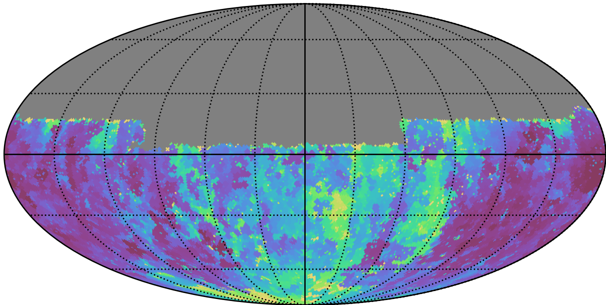
weather_cloudso4v3.4_10yrs Yr 1 u band: Min seeingGeom
