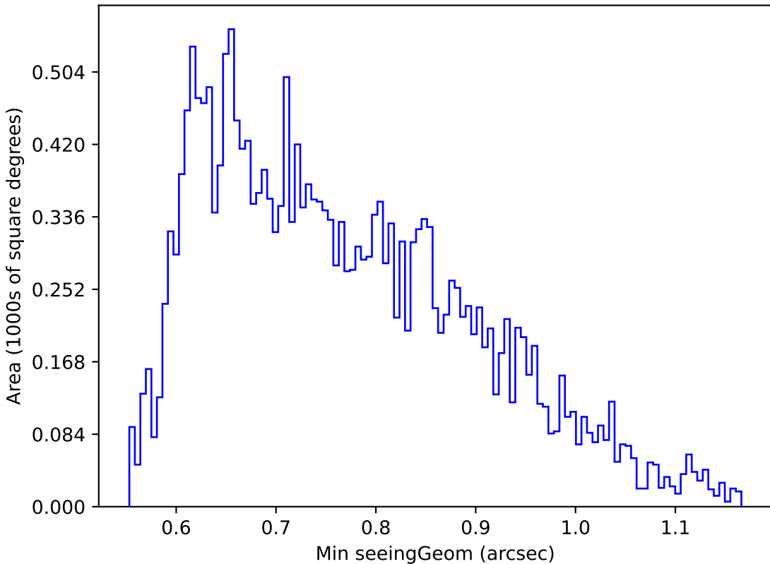
weather_cloudso4v3.4_10yrs Yr 1 u band: Min seeingGeom
