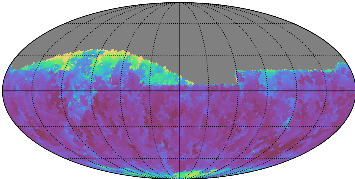
weather_cloudso4v3.4_10yrs Yr 1 i band: Min seeingGeom
