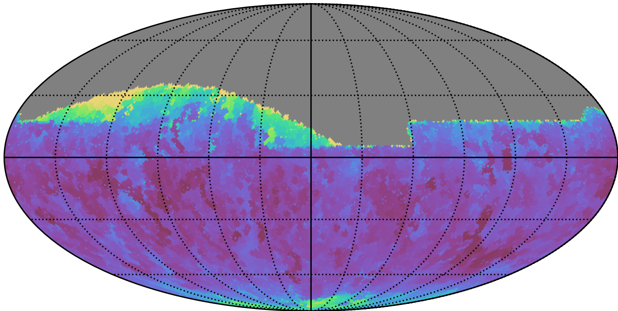
weather_cloudso4v3.4_10yrs Yr 1 all bands: Min seeingGeom
