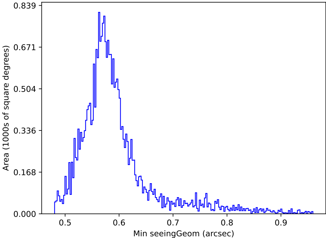
weather_cloudso4v3.4_10yrs Yr 1 all bands: Min seeingGeom
