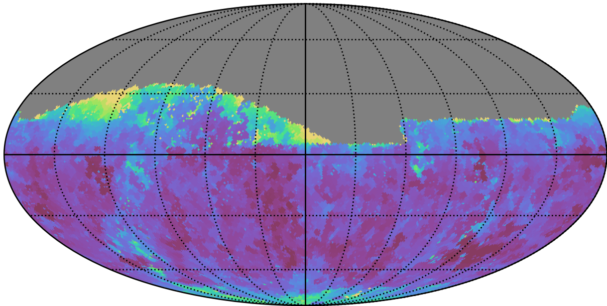
weather_cloudso4v3.4_10yrs Yr 1 z band: Min seeingEff
