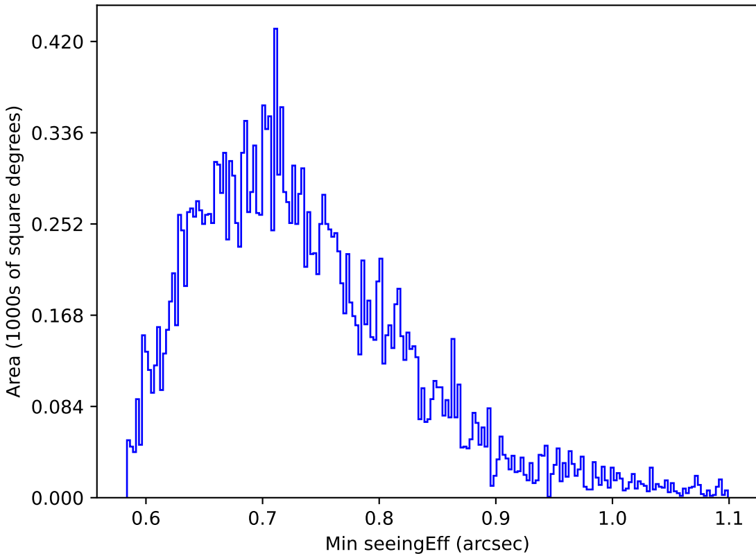
weather_cloudso4v3.4_10yrs Yr 1 y band: Min seeingEff
