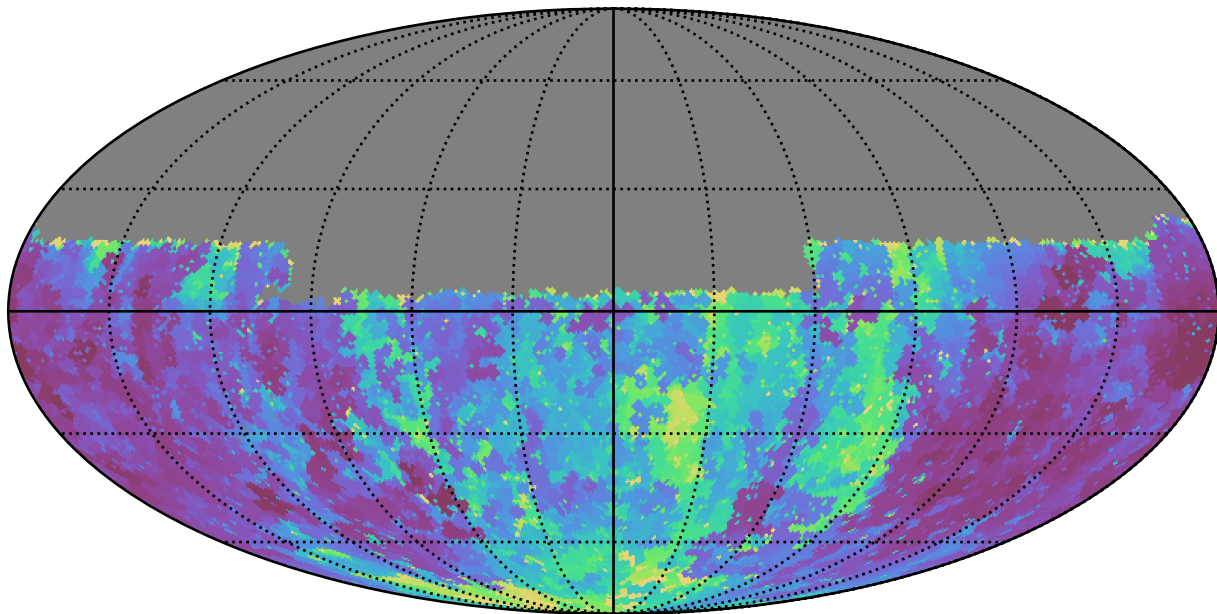
weather_cloudso4v3.4_10yrs Yr 1 u band: Min seeingEff
