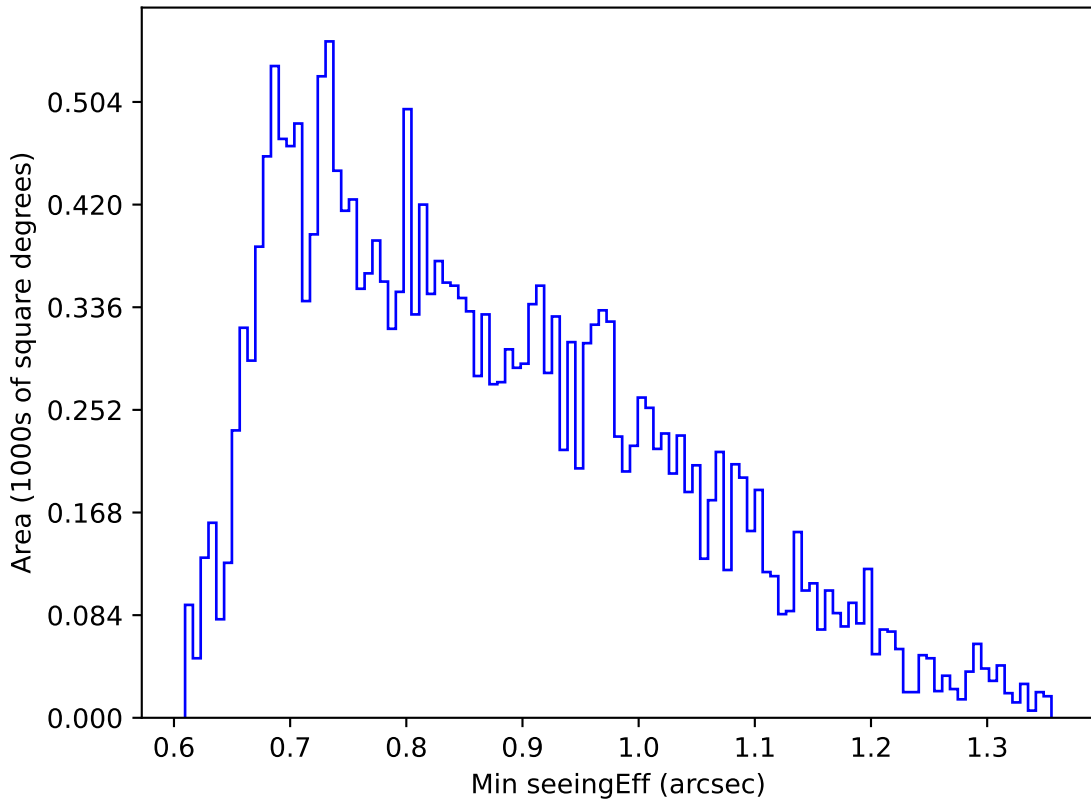
weather_cloudso4v3.4_10yrs Yr 1 u band: Min seeingEff
