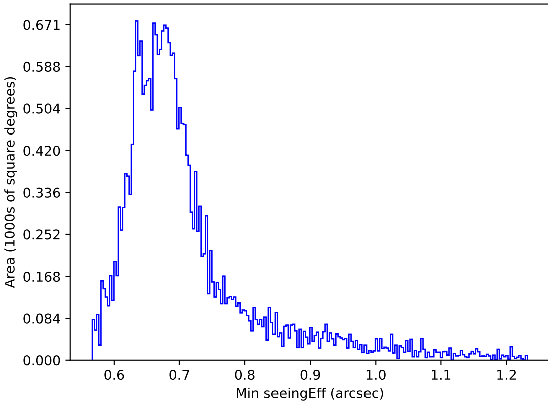
weather_cloudso4v3.4_10yrs Yr 1 i band: Min seeingEff
