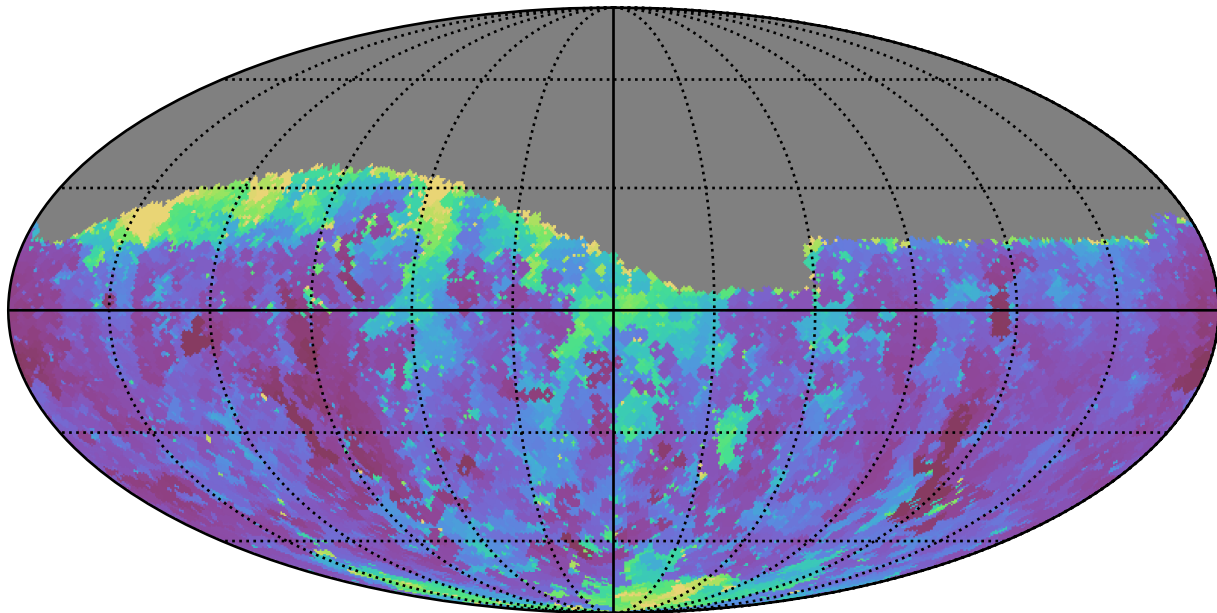
weather_cloudso4v3.4_10yrs Yr 1 g band: Min seeingEff
