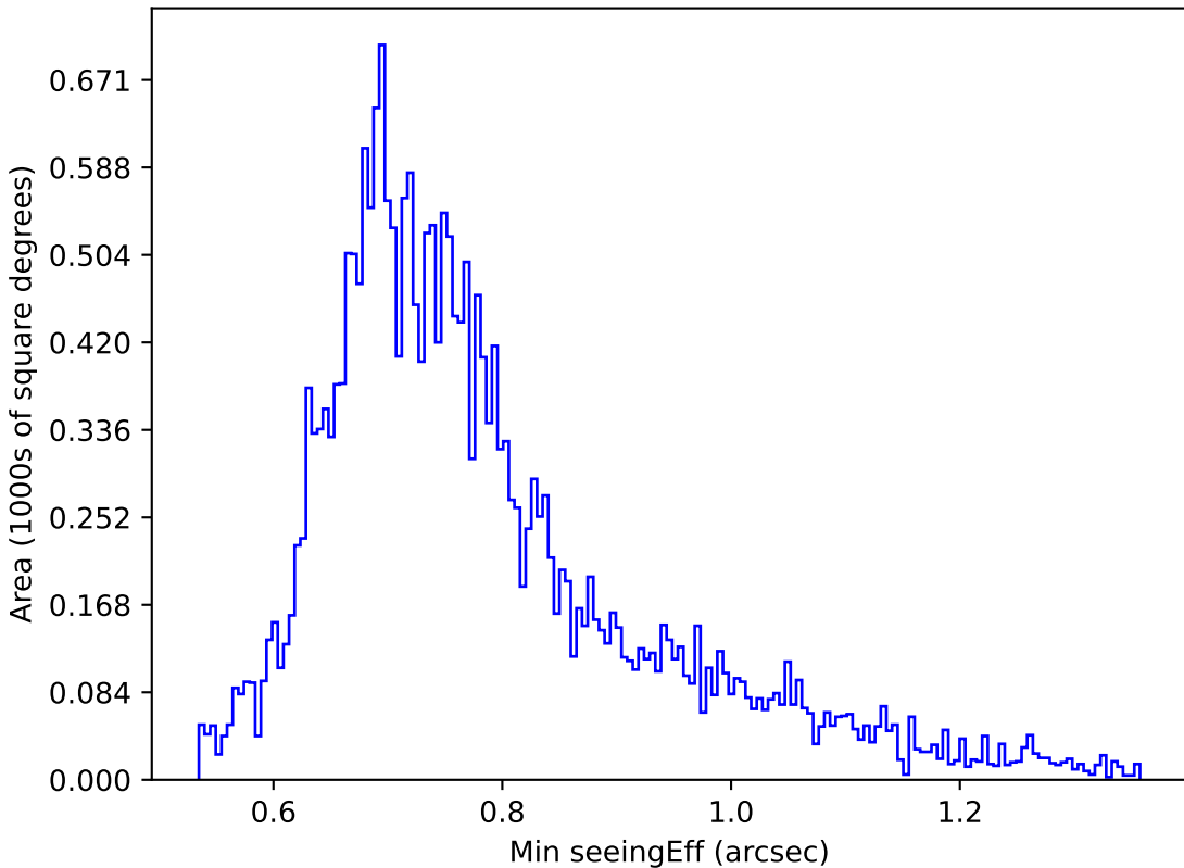
weather_cloudso4v3.4_10yrs Yr 1 g band: Min seeingEff
