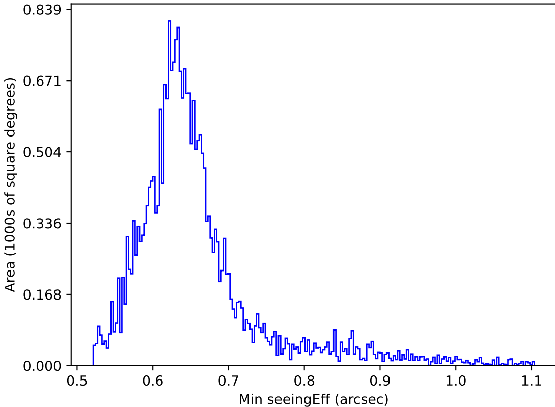
weather_cloudso4v3.4_10yrs Yr 1 all bands: Min seeingEff
