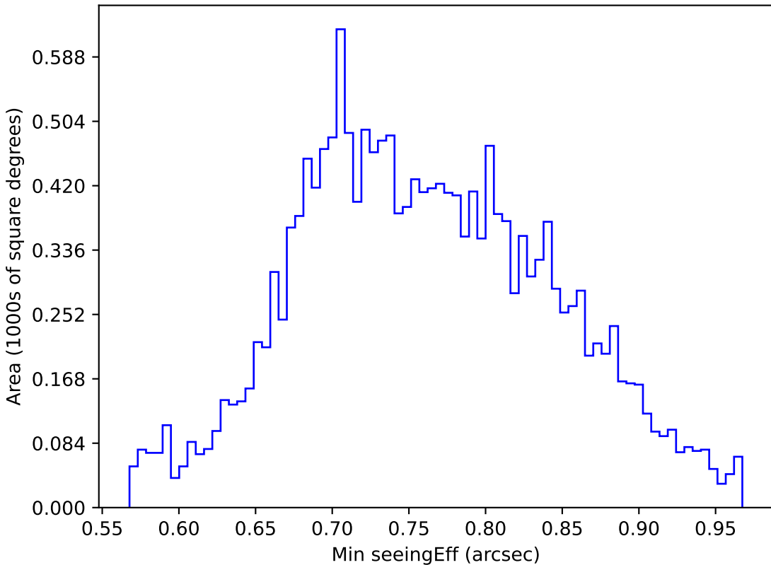
weather_cloudso4v3.4_10yrs WFD u band: Min seeingEff
