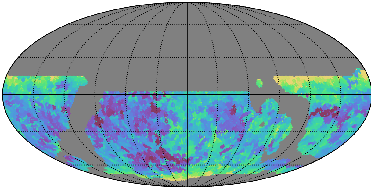
weather_cloudso4v3.4_10yrs WFD r band: Min seeingEff
