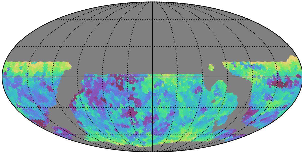
weather_cloudso4v3.4_10yrs WFD i band: Min seeingEff
