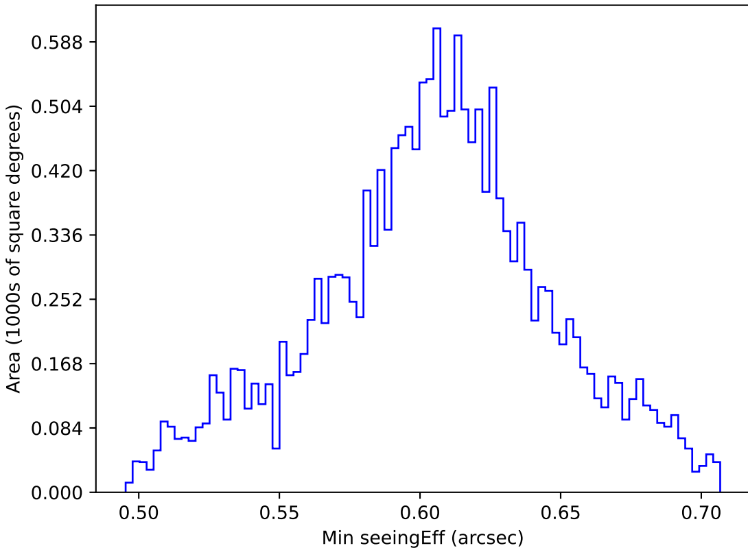
weather_cloudso4v3.4_10yrs WFD i band: Min seeingEff
