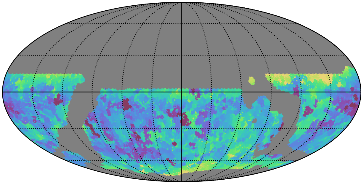
weather_cloudso4v3.4_10yrs WFD g band: Min seeingEff
