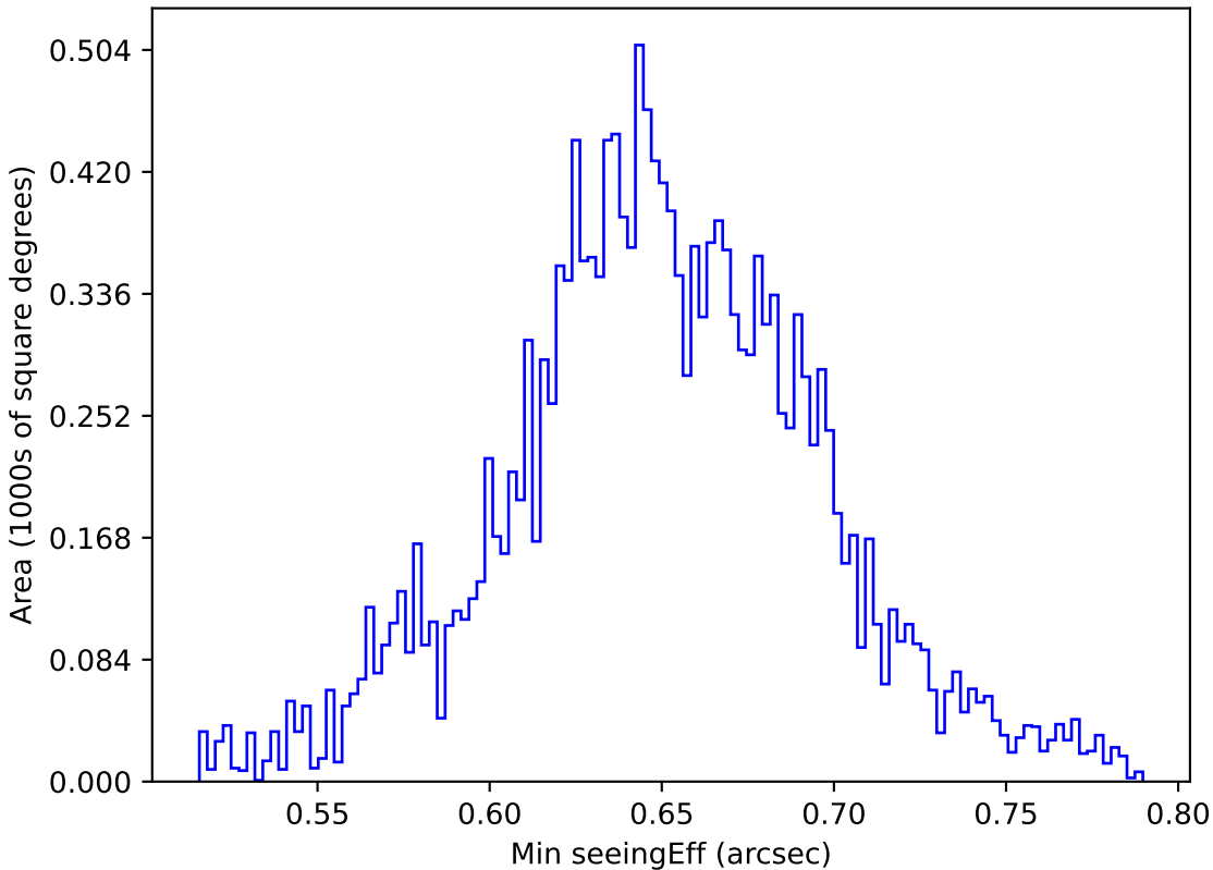
weather_cloudso4v3.4_10yrs WFD g band: Min seeingEff
