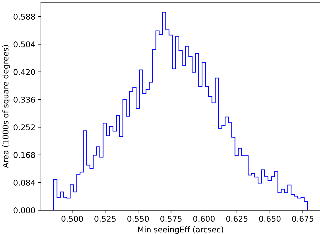
weather_cloudso4v3.4_10yrs WFD all bands: Min seeingEff
