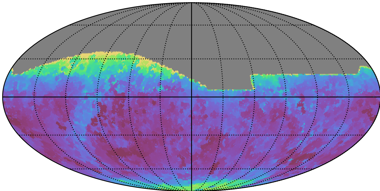
weather_cloudso4v3.4_10yrs All sky z band: Min seeingEff
