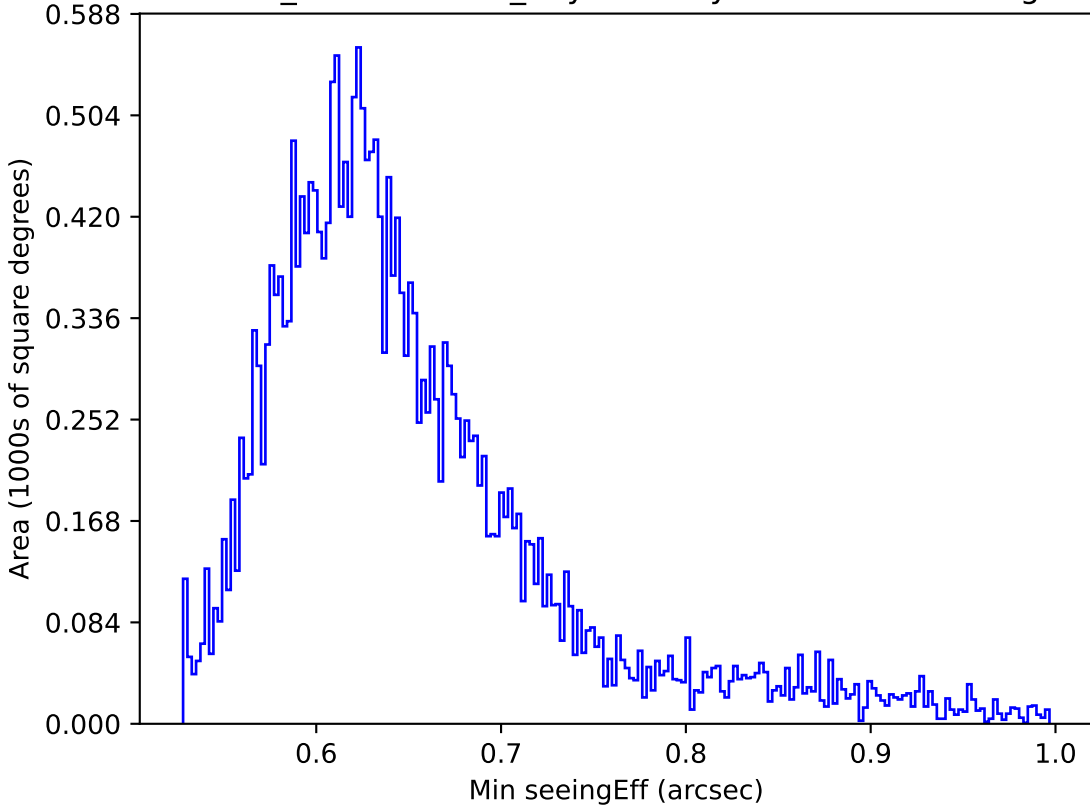
weather_cloudso4v3.4_10yrs All sky z band: Min seeingEff
