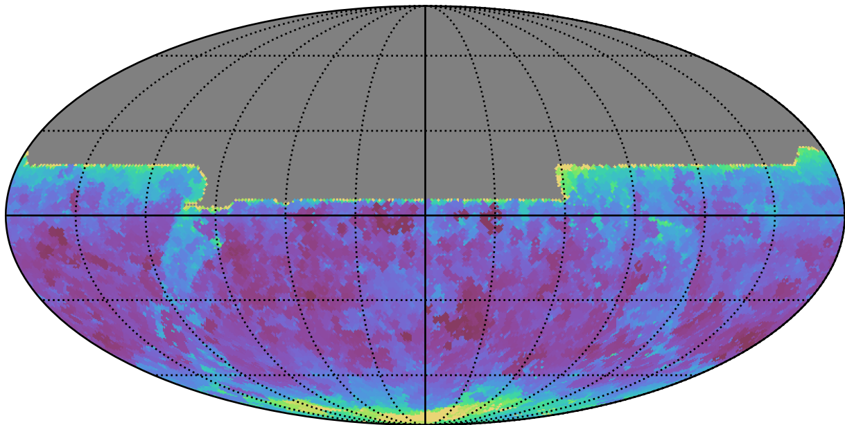
weather_cloudso4v3.4_10yrs All sky y band: Min seeingEff
