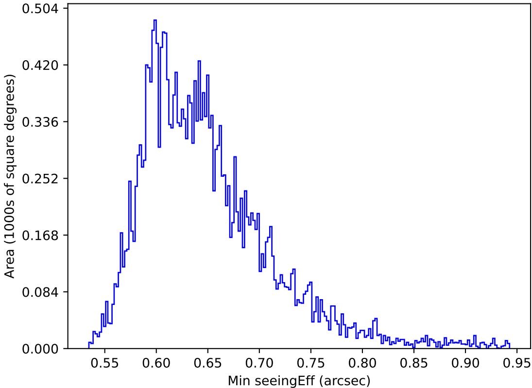
weather_cloudso4v3.4_10yrs All sky y band: Min seeingEff
