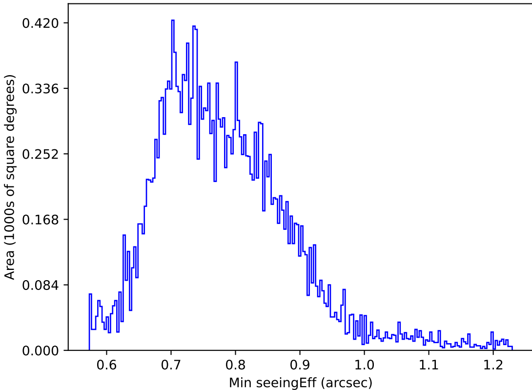
weather_cloudso4v3.4_10yrs All sky u band: Min seeingEff
