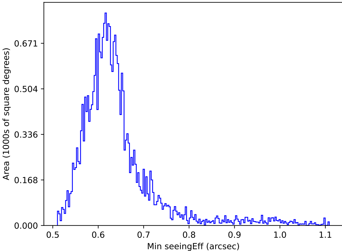
weather_cloudso4v3.4_10yrs All sky r band: Min seeingEff
