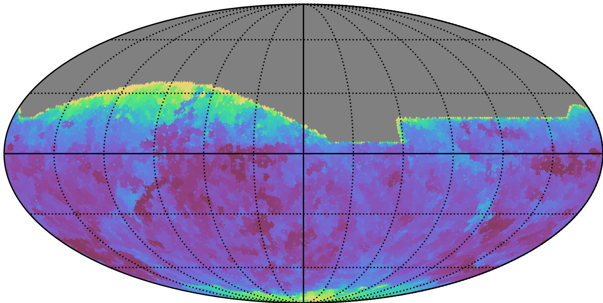
weather_cloudso4v3.4_10yrs All sky i band: Min seeingEff
