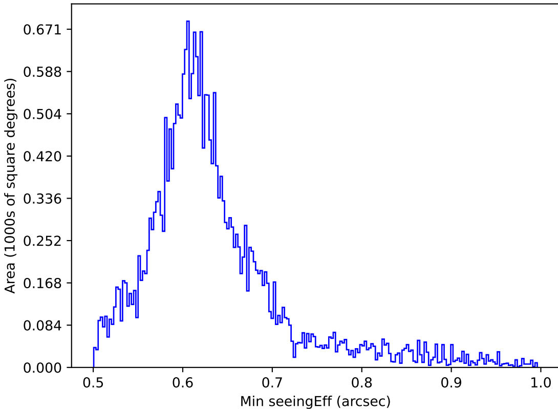
weather_cloudso4v3.4_10yrs All sky i band: Min seeingEff
