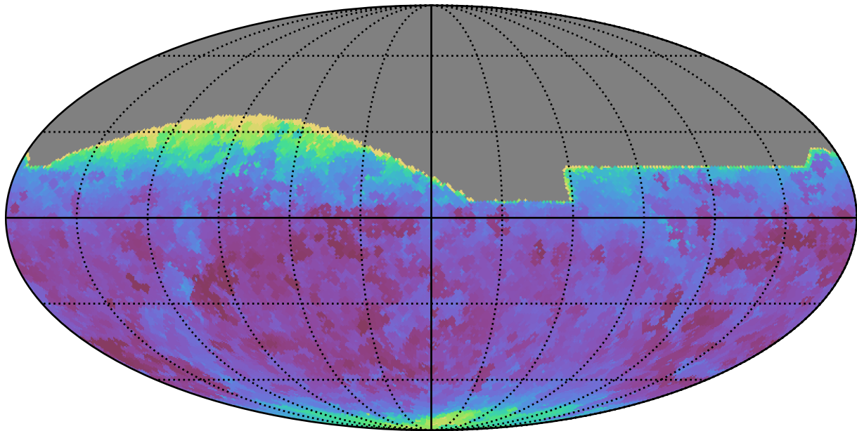
weather_cloudso4v3.4_10yrs All sky all bands: Min seeingEff
