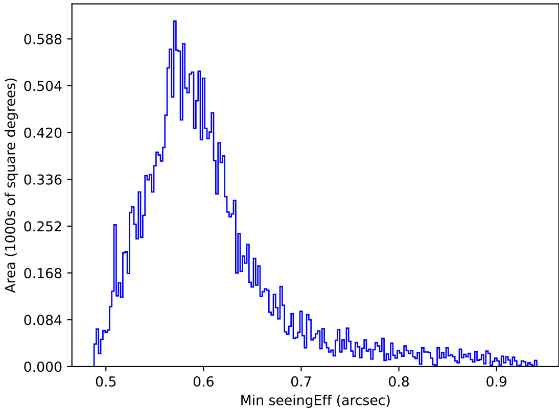
weather_cloudso4v3.4_10yrs All sky all bands: Min seeingEff
