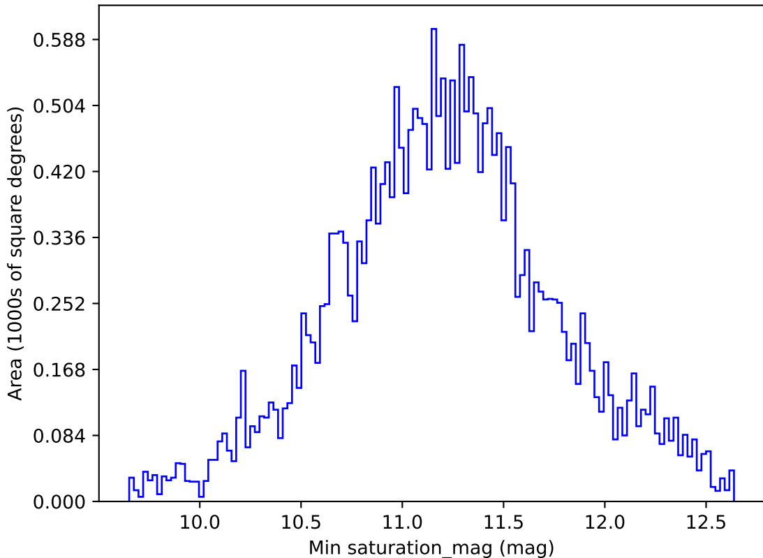
weather_cloudso4v3.4_10yrs All sky all bands: Min saturation_mag
