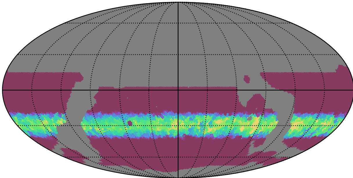
weather_cloudso4v3.4_10yrs WFD z band: Min normairmass
