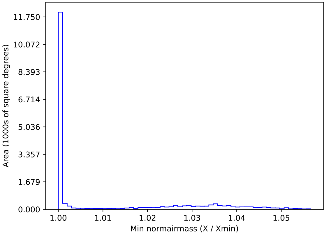
weather_cloudso4v3.4_10yrs WFD u band: Min normairmass
